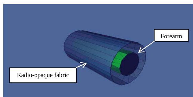
Figure 1: Forearm model geometry. The green cylindrical surface represents the forearm tissue, while the darker blue cylindrical surface represents the layers of radio-opaque fabric. Note that the radio-opaque fabric is modelled in three distinct layers; however, two of them are too small to be seen in the figure.
