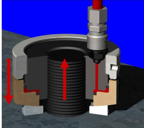
Figure 5: Resultant pre load stretches the stud and compresses the flange
