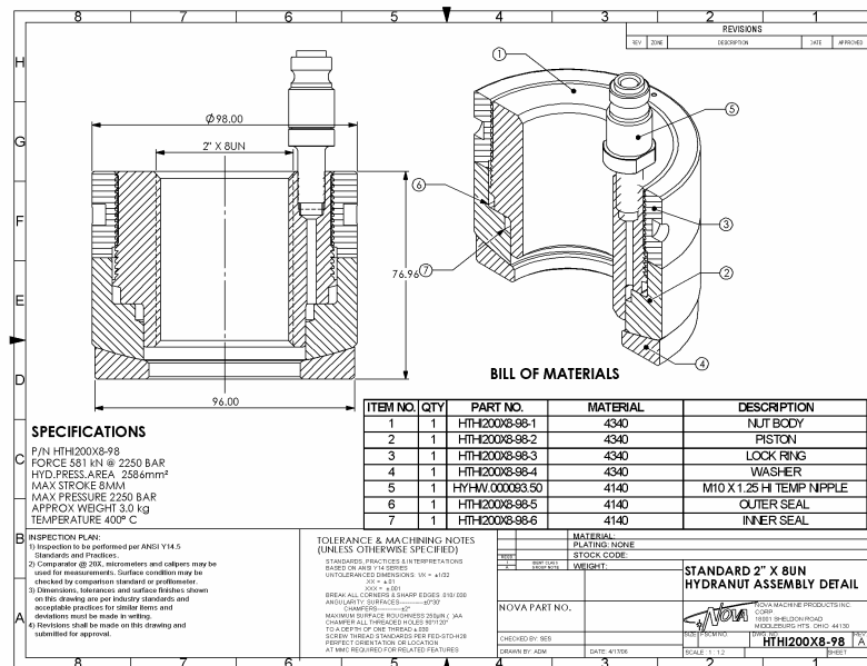
Figure 1 – Typical Hydraulic Nut assembly
