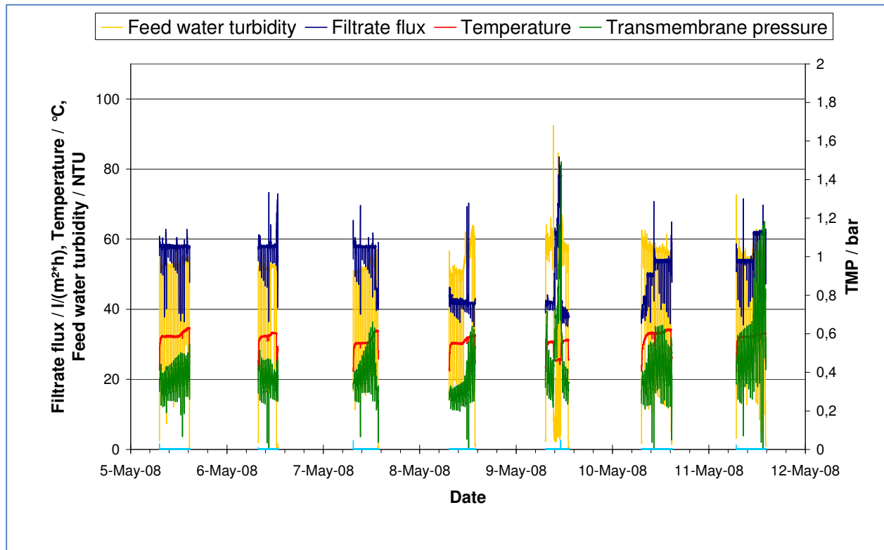
Figure 3 – Pilot trial - parameters from May 5 – 12
