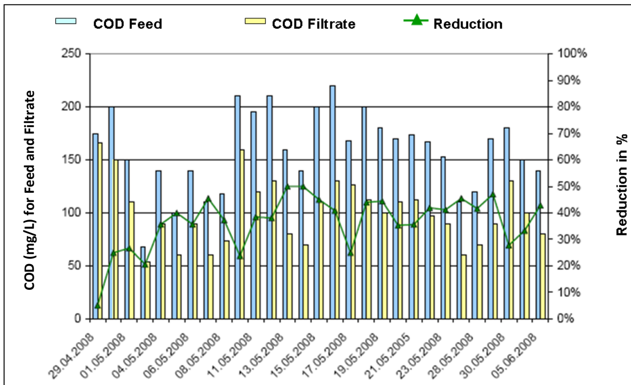
Figure 5 – Chemical Oxygen Demand (COD) reduction
