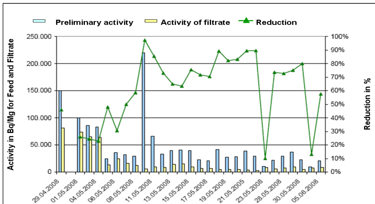
Figure 4 – Radioactive material reduction
