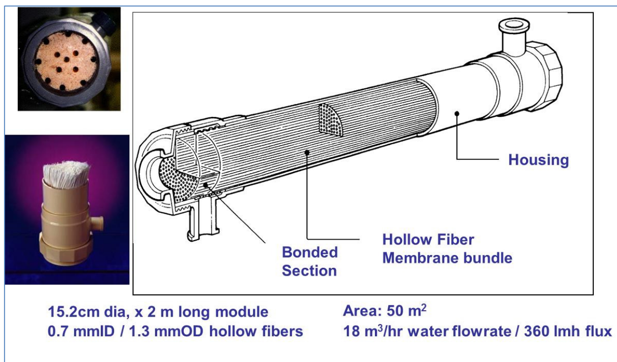
Figure 1 - Hollow Fiber Microfiltration Module
