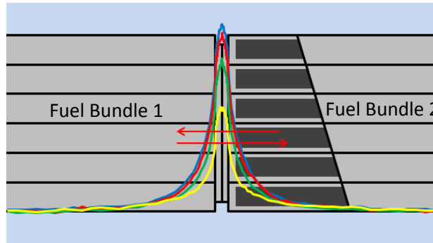
Figure 1: End Flux Peaking is created due to trapping of thermal neutrons, from all sources, in the end regions, see Figure 2 for detailed description of the end region of a fuel bundle
