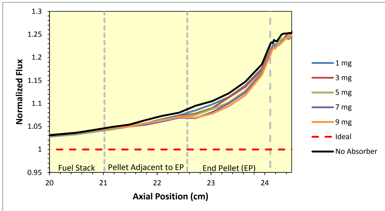
Figure 5: Preliminary absorber trials with europium placed with the end pellet
