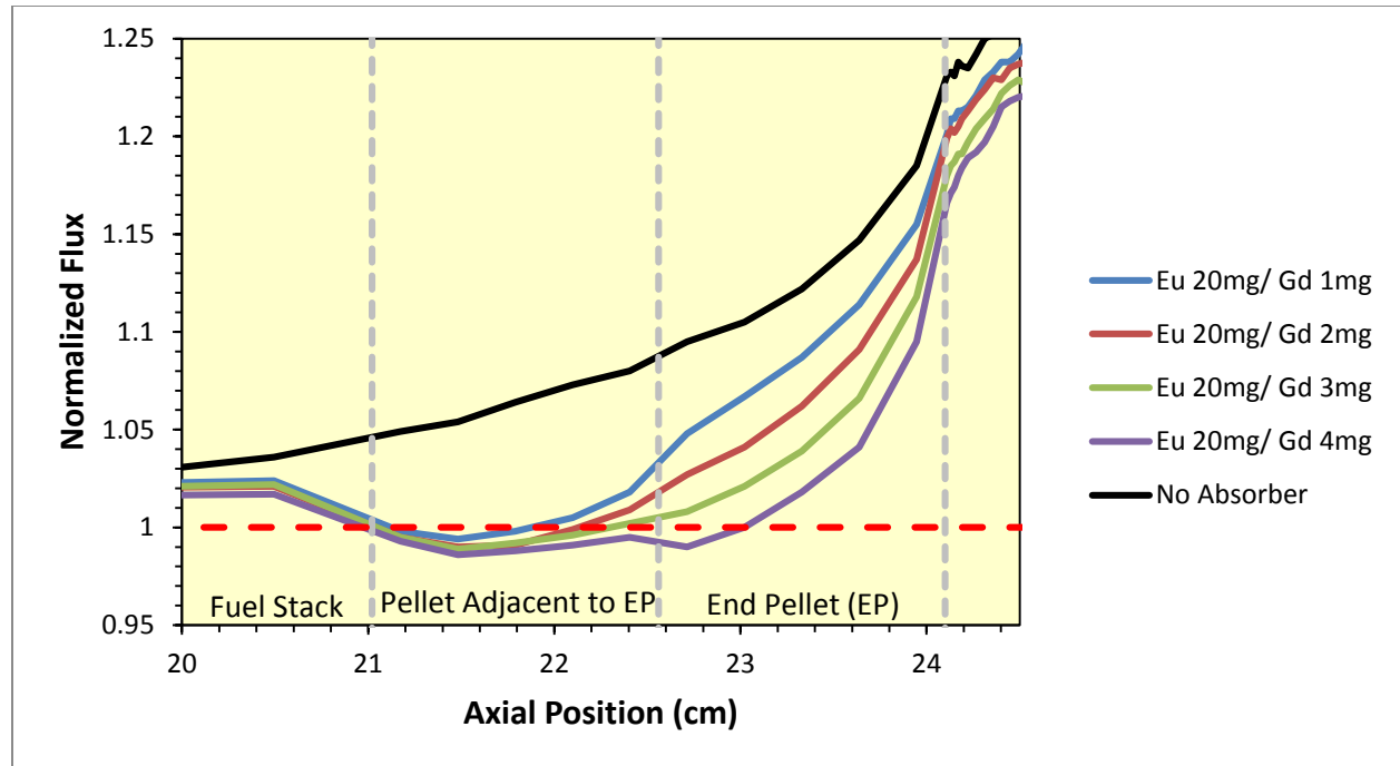
Figure 7: Absorber trials with europium placed within the pellet adjacent to the end pellet and gadolinium placed within the end pellet.
