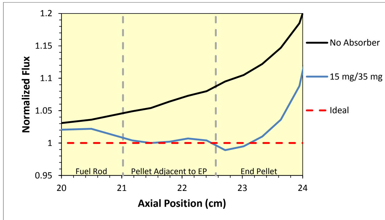
Figure 8: Comparing the ideal europium trials with the case of having no absorber
