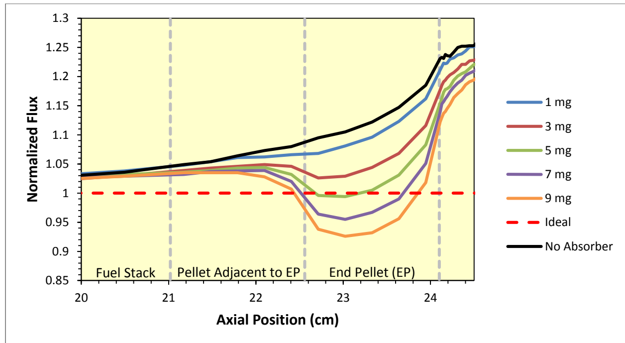
Figure 3: Preliminary absorber trials with various amounts of gadolinium placed in the end pellet, for values greater than 24 cm we get into the end cap/plate where peaking factor is of less concern.
