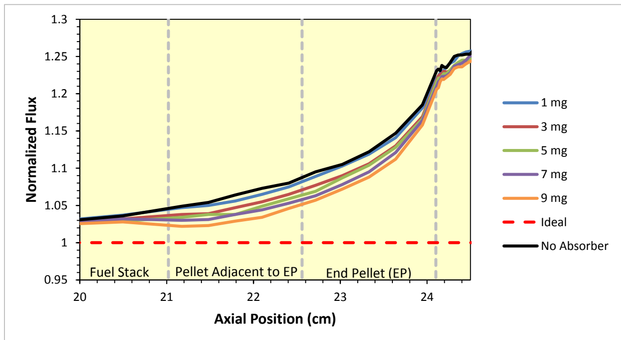
Figure 6: Preliminary absorber trials with europium placed in both the end pellet and the pellet adjacent to the end pellet, same amount in each pellet
