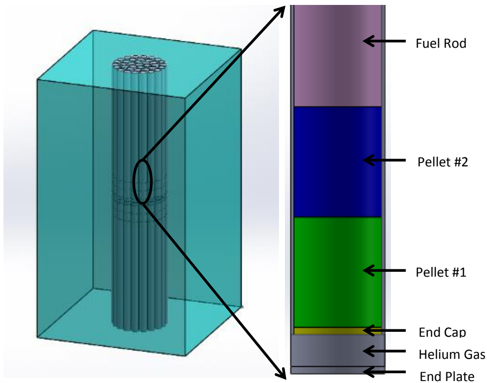
Figure 2: Two half CANDU bundle model, including blown up cross section of a fuel element
