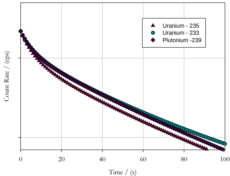
Figure 3: Time Dependant Delayed Neutron Counts for SNMs U-233, U-235 and Pu-239 Normalized to Equal t=0 Counts.
