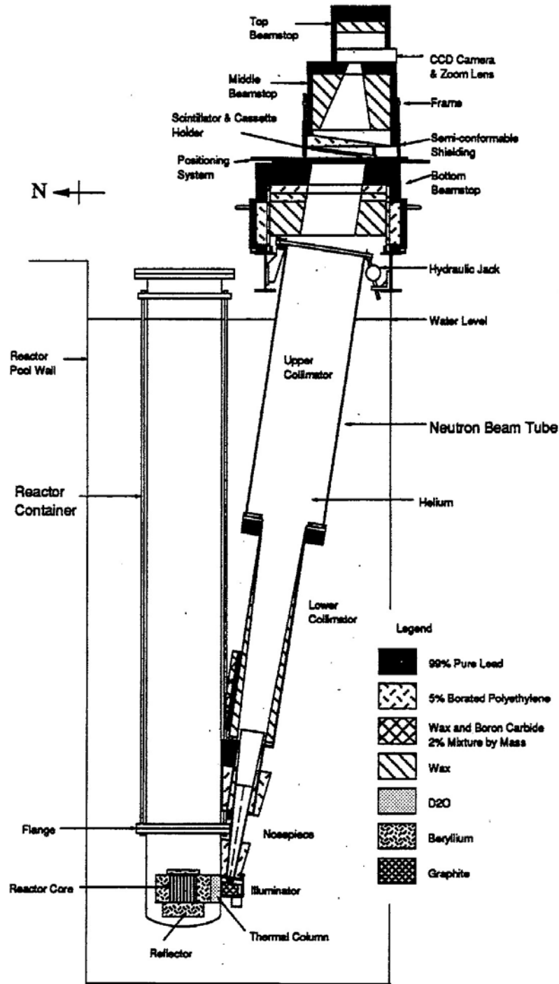
Figure 2 : Side View of RMCC Neutron Imaging System
