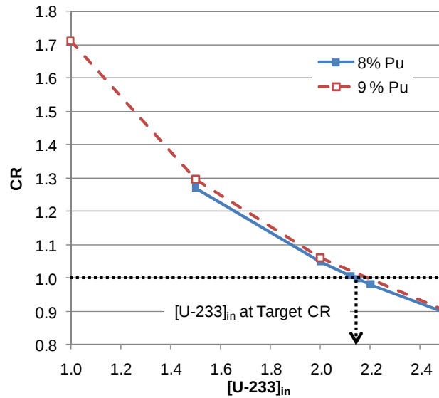
Figure 8 CR versus input [U-233] for 24 cm LP
