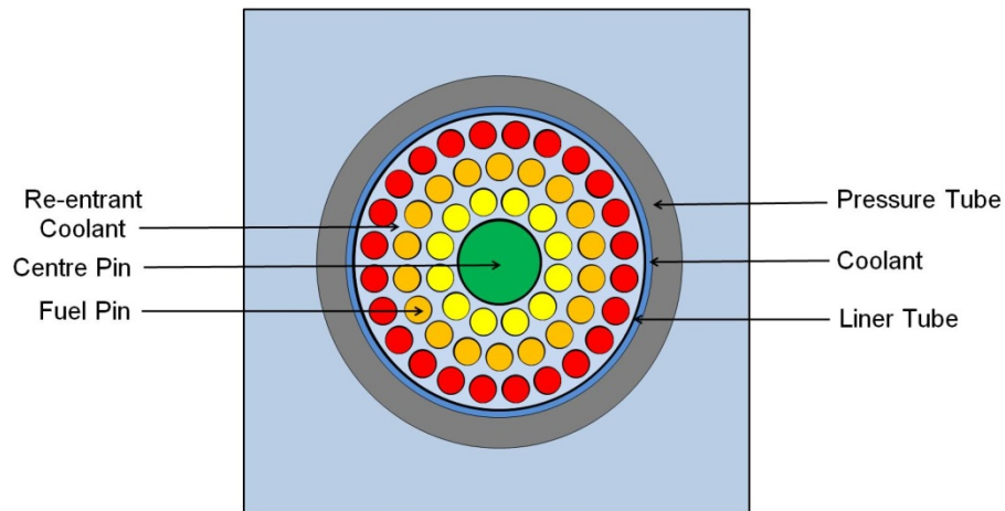
Figure 1 SCWR 54-Element Bundle Design and Re-entrant channel (REC) lattice cell
