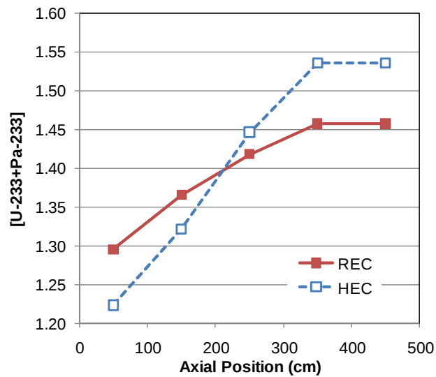
Figure 6 Final [U-233+Pa-233] versus axial position
