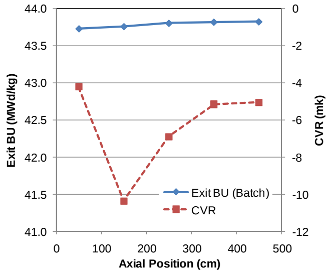
Figure 11 Exit Burnup and CVR versus Axial Position (HEC)
