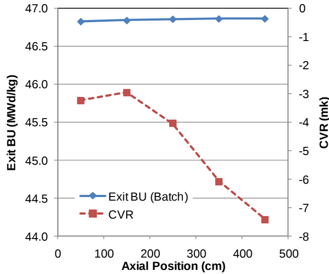
Figure 10 Exit Burnup and CVR versus Axial Position (REC)
