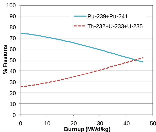
Figure 13 Percent Fissions from Pu-derived and Th-232-derived isotopes (REC)
