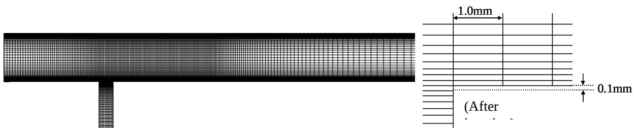
Figure 5 Mesh arrangement
