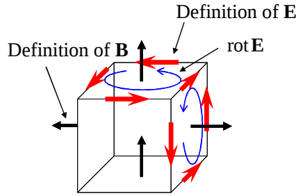
Figure 2 Staggered layout in control volume
