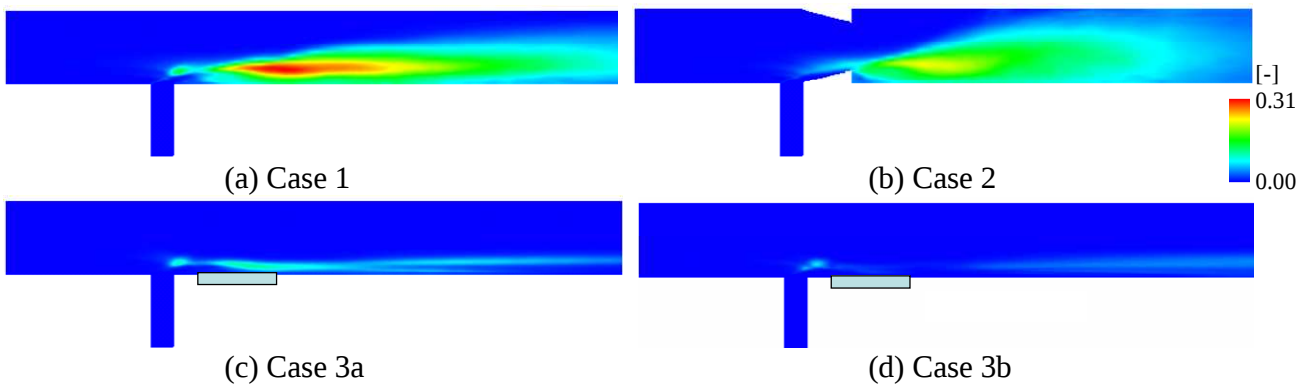
Figure 9 Distribution of temperature fluctuation
