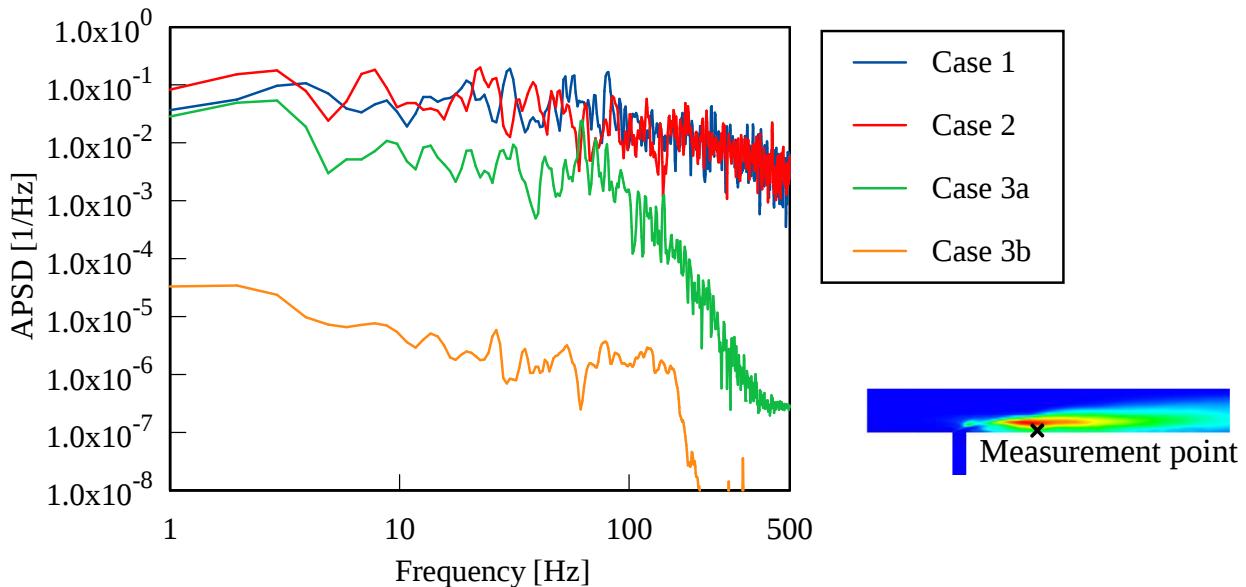
Figure 10 Auto-power spectrum density of reduced temperature
