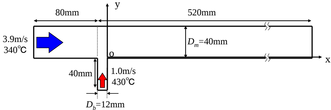
Figure 4 Analytical domain
