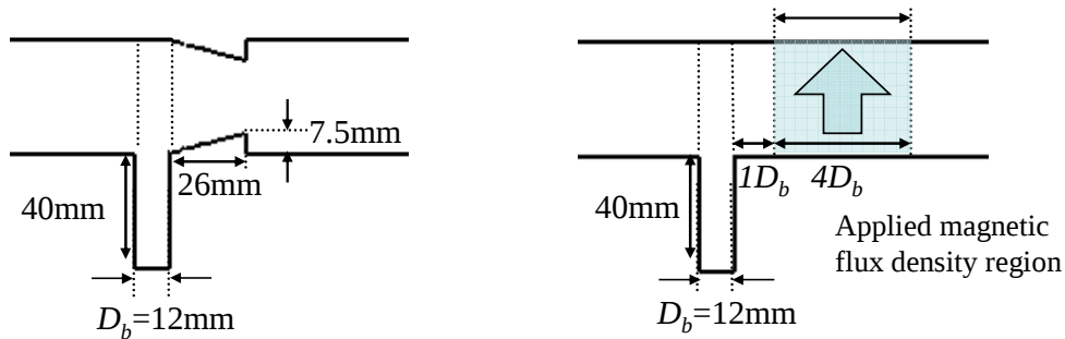
(a) Turbulence promoter (b) Applied magnetic flux density Figure 6 Additional installations for temperature mixing mitigation
