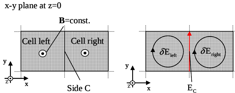
Figure 3 Schematic of electric intensity field corrector
