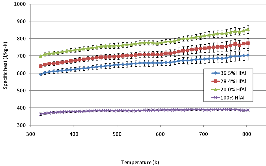
Figure 4 Specific heat of hafnium aluminide materials.
