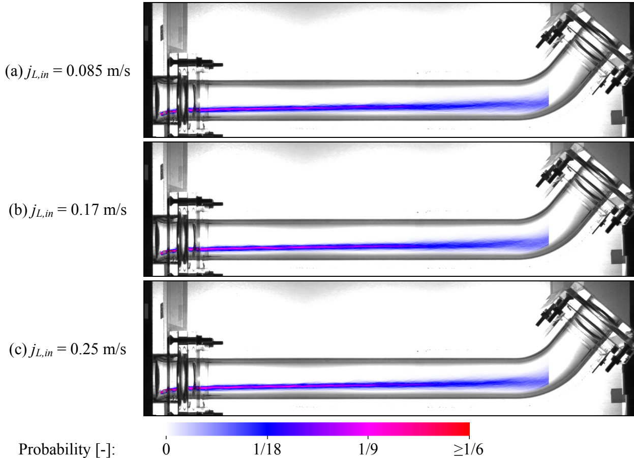
Figure 9 Evolution of the probability distribution of the water level in function of the injected water flow rate for experiments with j_G = 4.0 m/s.
