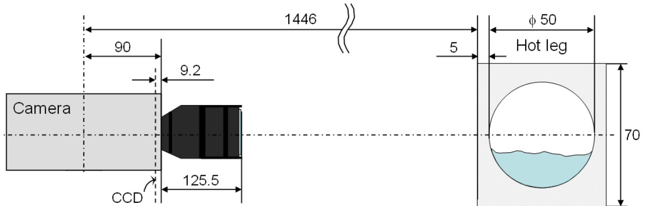
Figure 2 Cross section of the hot leg pipe and position of the camera.
