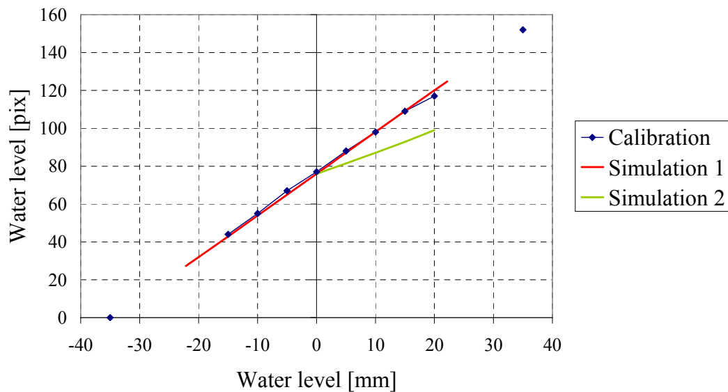
Figure 4 Vertical resolution of the optical observation: comparison between experimental calibration and simulation
