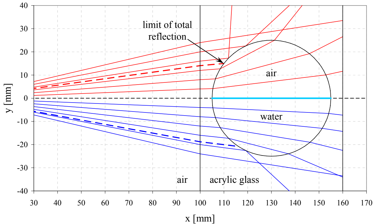
Figure 3 Scheme of the simulated optical path through the hot leg cross-section (distance between camera and channel outer wall: 100 mm).
