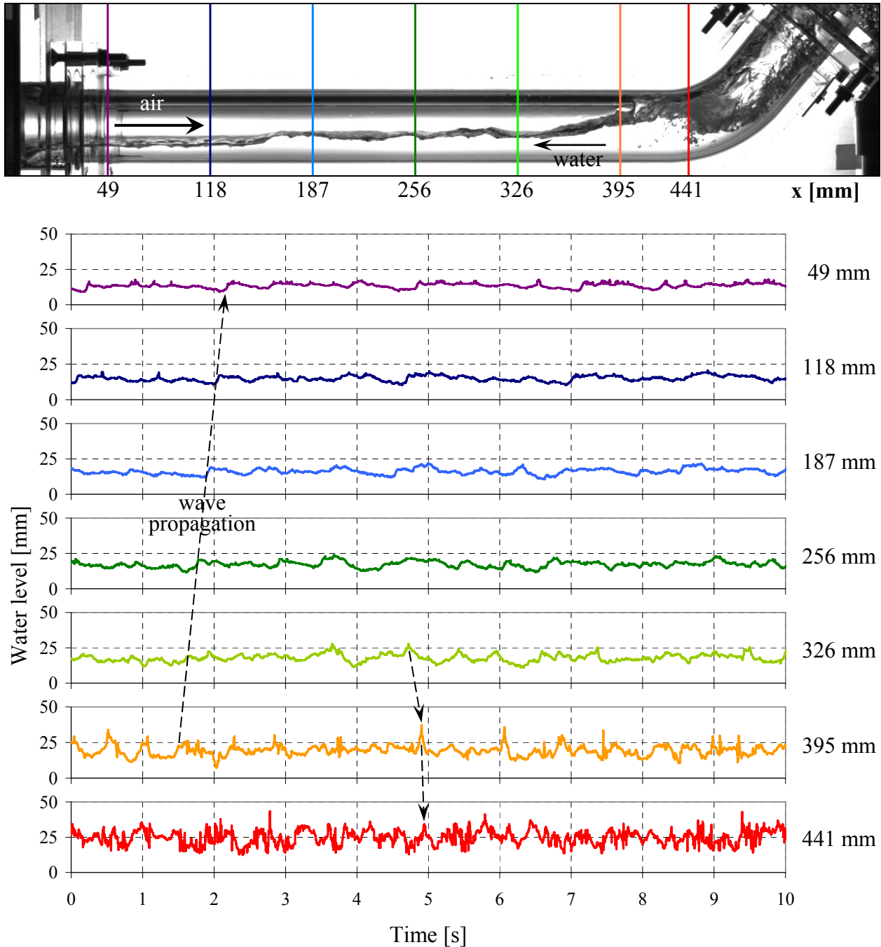
Figure 6 Time-dependent water level in chosen cross-sections during CCFL at j_{L,in} = 0.25 m/s and j_G = 4.0 m/s.
