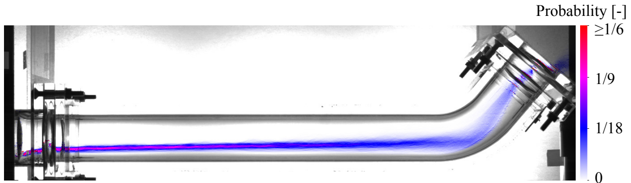
Figure 7 Visualisation of the probability distribution of the water level (colours) over the background picture (black and white) – CCFL at j_{L,in} = 0.25 m/s and j_G = 4.0 m/s.
