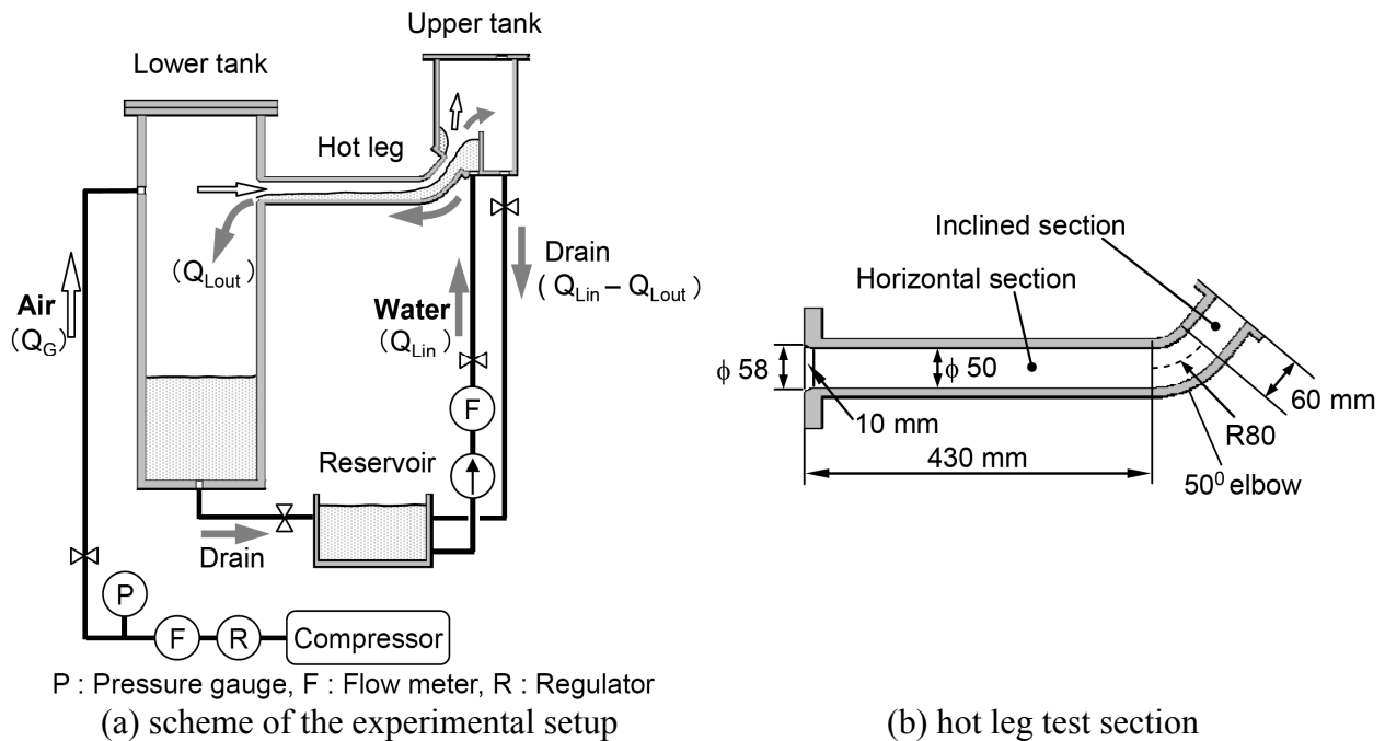
Figure 1 Hot leg test facility of Kobe University.
