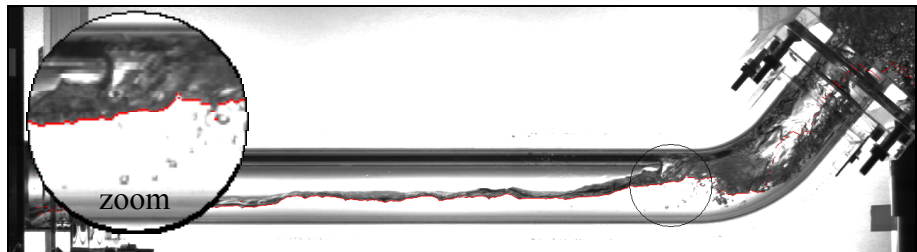
Figure 5 Visualisation of the main steps of the image processing (image taken during CCFL at j_{L,in} = 0.25 m/s and j_G = 4.0 m/s).
