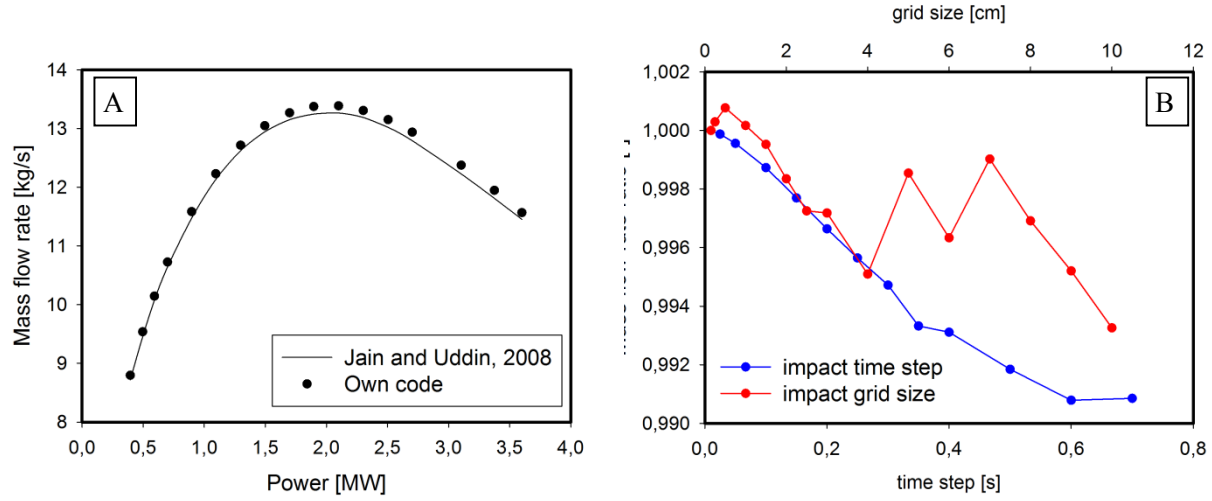
Figure 5: A: comparison of the simulated power-flow to data by Jain and Uddin [19], B: grid and time step independence study for DeLight model (5kW, T_{in} : 0°C)
