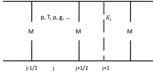
Figure 4. Discretization grid.
