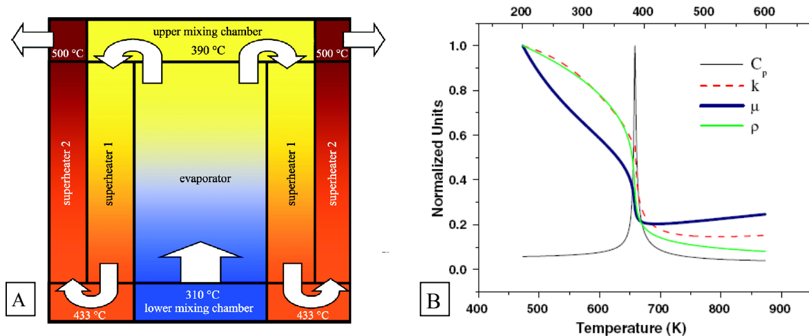
Figure 1. A: Three pass core arrangement proposed for the HPLWR (Fischer et al. [9]), B: normalized fluid properties (specific heat capacity C_p , thermal conductivity k , dynamic viscosity \eta and density \rho ) for water at 25 MPa for a range of temperatures
