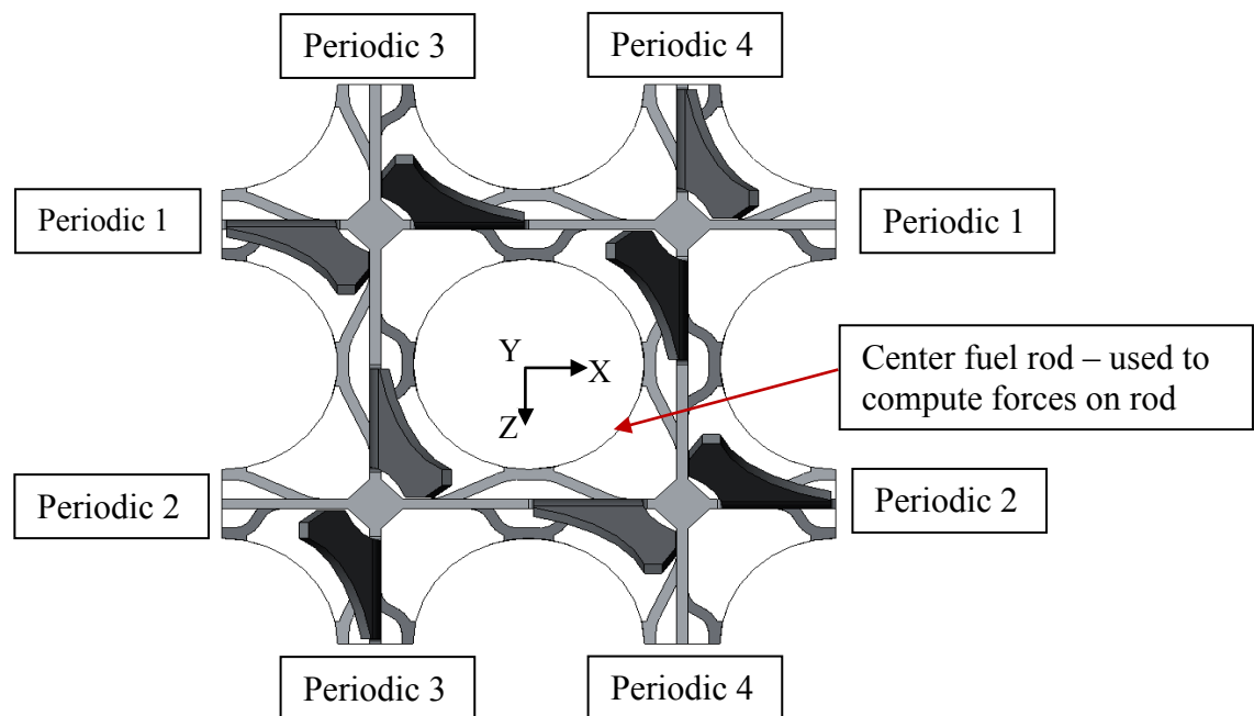
Figure 1: Grid Geometry and Periodic Boundary Conditions Used in the CFD Model
