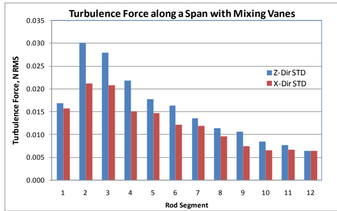
Figure 7: Excitation force distribution along a span – Grid with mixing vanes
