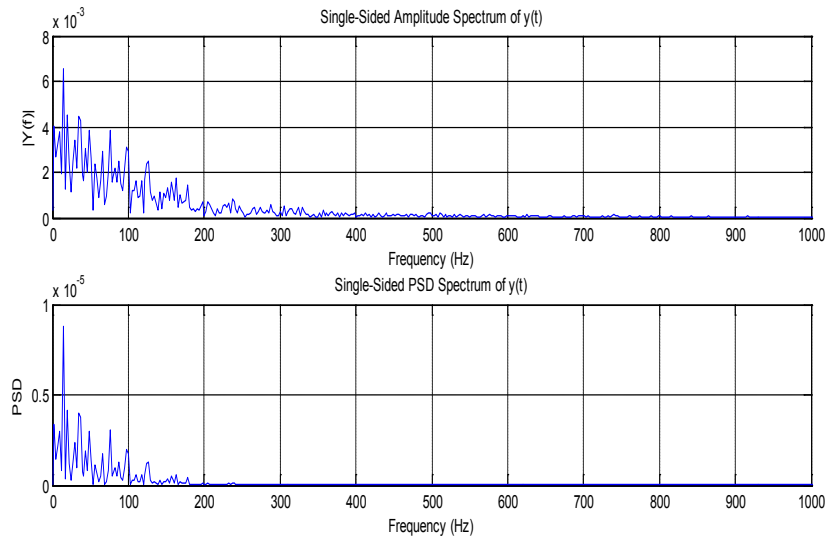
Figure 10: FFT amplitude and PSD spectrum – Segment 2
