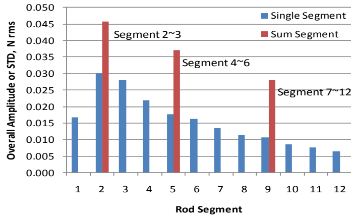
Figure 12: Segment forces and lumped forces
