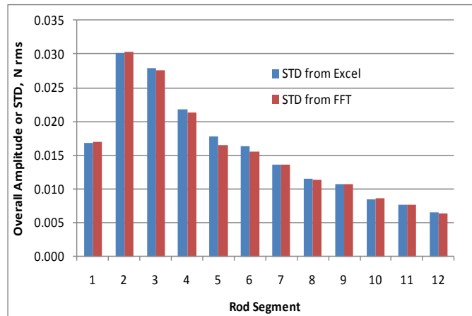
Figure 9: Standard Deviation comparison of Excel and FFT code
