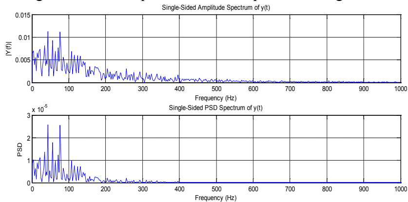
Figure 11: FFT amplitude and PSD spectrum – Segment 7
