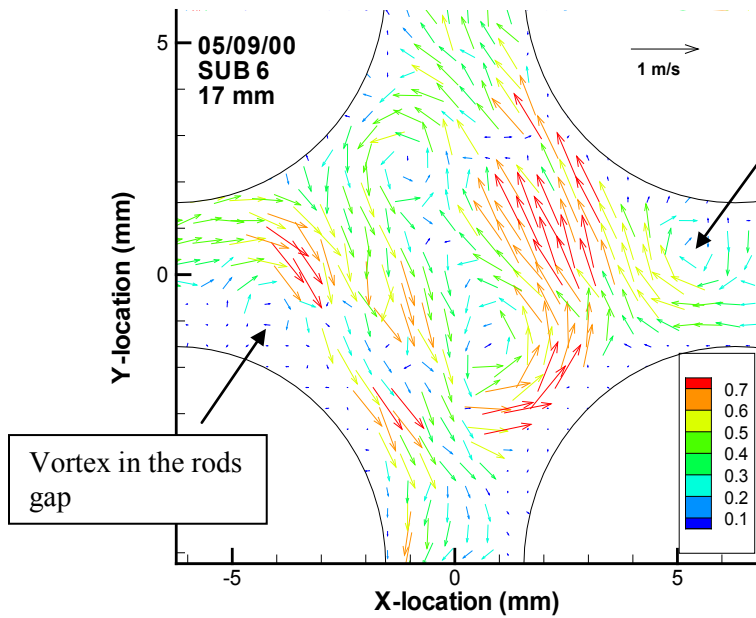
Figure 5 (a) Lateral velocity vectors from PIV data at 0.67 inch above strap
