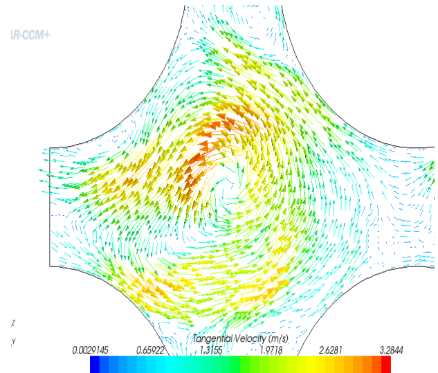
Figure 6 (a) Lateral velocity vectors from CFD at 1.97 inch above grid strap
