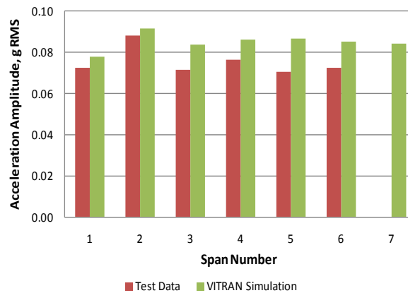
Figure 13: Fuel rod acceleration vibration amplitude: Test data vs. CFD/VITRAN simulation
