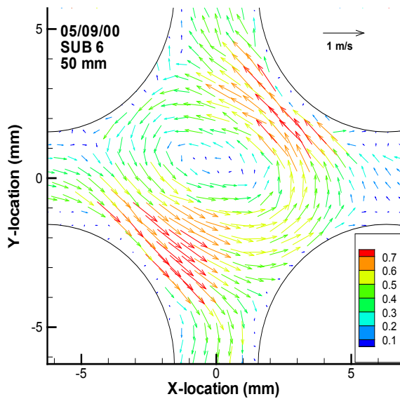
Figure 6 (a) Lateral velocity vectors from PIV at 1.97 inch above grid strap
