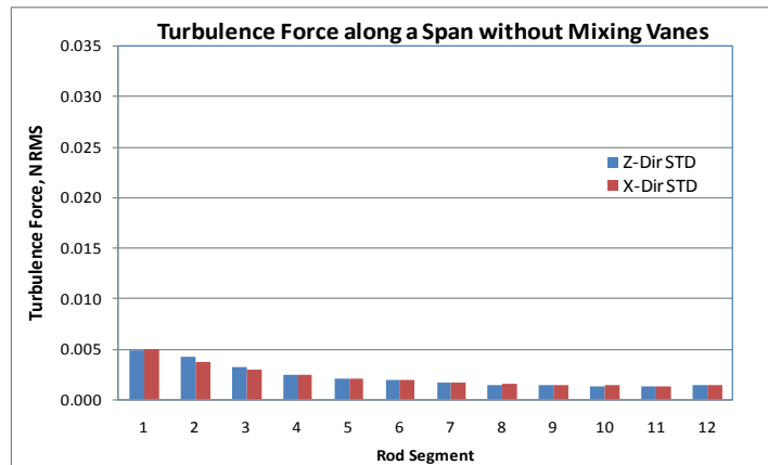
Figure 8: Excitation force distribution along a span – Grid without mixing vanes
