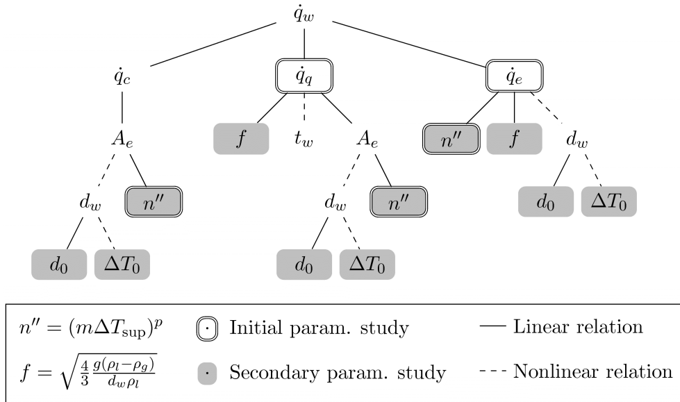
Figure 3. STAR-CD sub-cooled boiling model hierarchy
