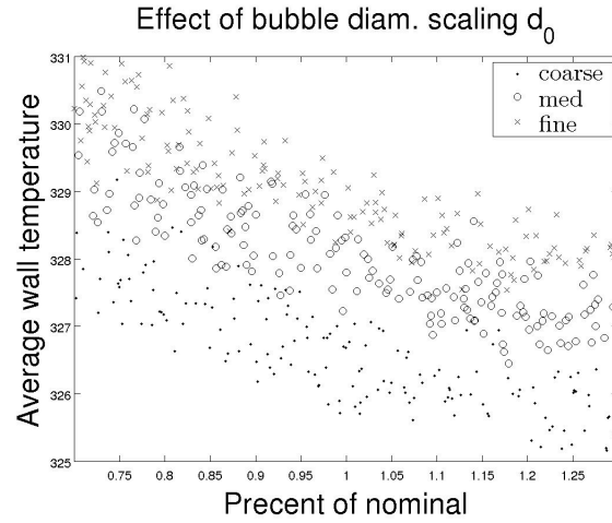
Figure 7. Effect of d_0 on average wall temperature
