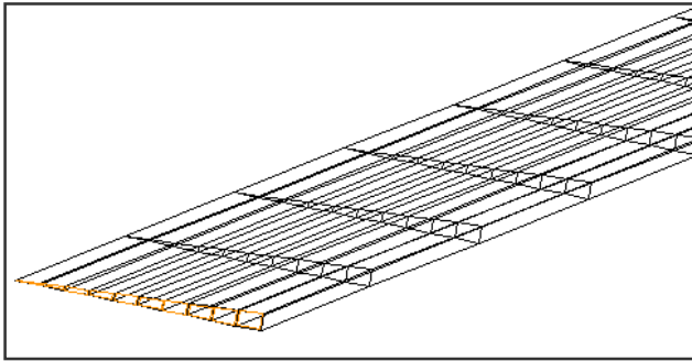
Figure 1. Portion of the mesh used in the STAR-CD model
