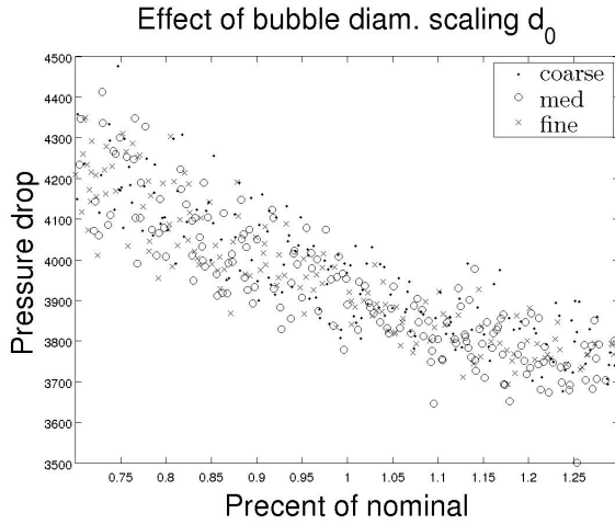
Figure 6. Effect of d_0 on pressure drop
