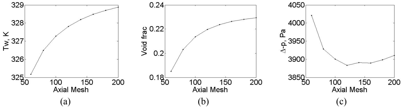
Figure 4. Mesh sensitivity of (a) average wall temperature, (b) void fraction at end of heated section, and (c) pressure drop across pipe.
