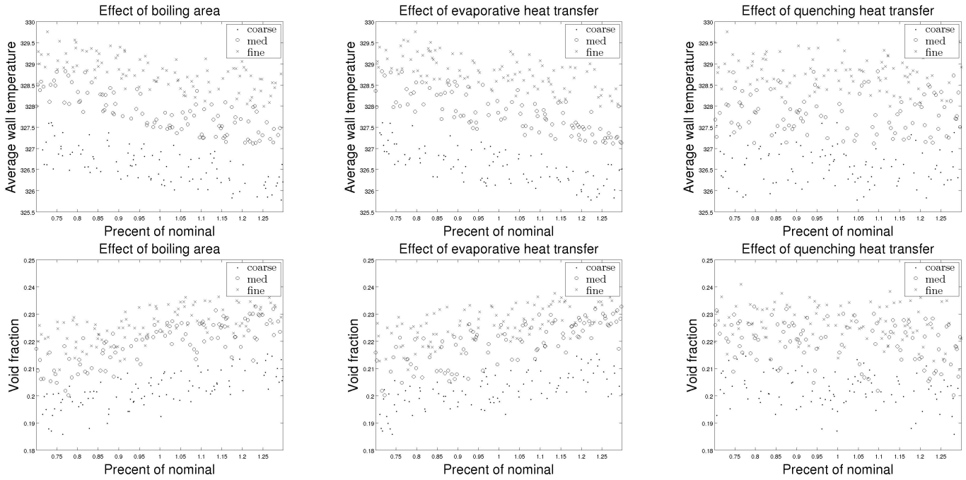
Figure 5. Sensitivity of outputs to boiling area, evaporative heat transfer, and quenching heat transfer
