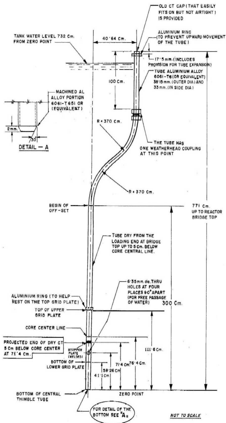
Figure 2 : Schematic drawing of Dry CT tube for I-131 production.
