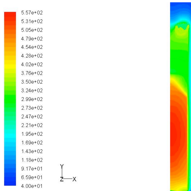
Figure 9 : Contours of static temperature ( °C)- Case-1: Dry CT tube with holes over the Al-can and the RNG k-\epsilon model.
