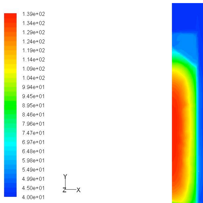
Figure 10 : Contours of static temperature ( °C) - Case-2 : Wet CT with holes over the Al-can and the RNG k-\epsilon model (Water Height : 2m).
