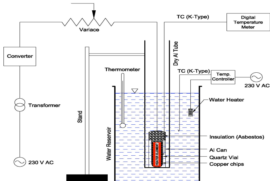
Figure 6 Schematic diagram of experimental set-up for Dry/Wet CT tube.
