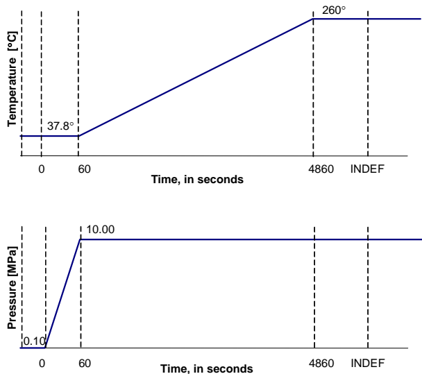
(a) Assumed Transient by Design
