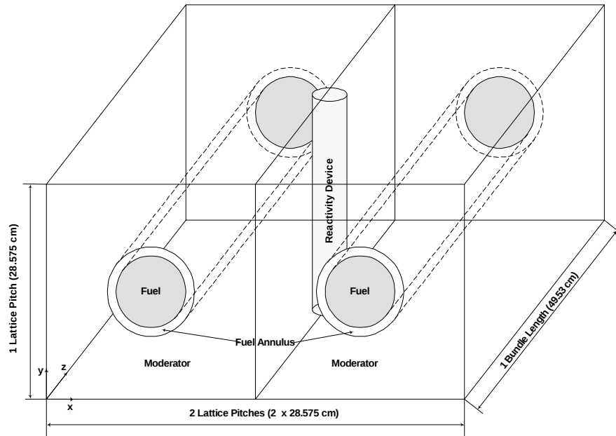
Figure 2 Homogenization Scheme
