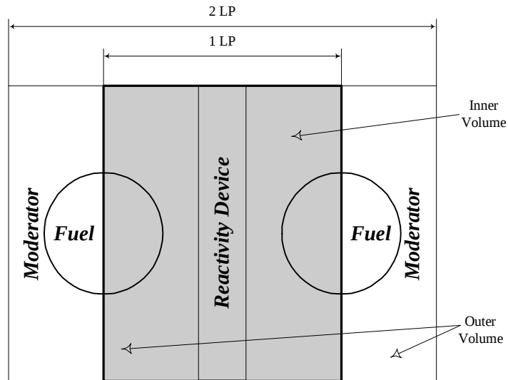
Figure 2 Homogenization Scheme
