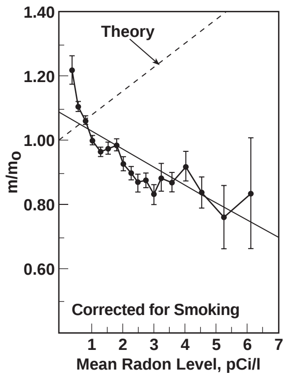
Figure 6. Lung cancer mortality rates compared with mean home radon levels by U.S. county and comparison with linear model by BEIR IV. m/m_0 = ratio of lung cancer mortality rate for residential radon levels to that at 0 level (theoretical), or to that at average residential level, 1.7 pCi/l. Cohen B, 1995.
