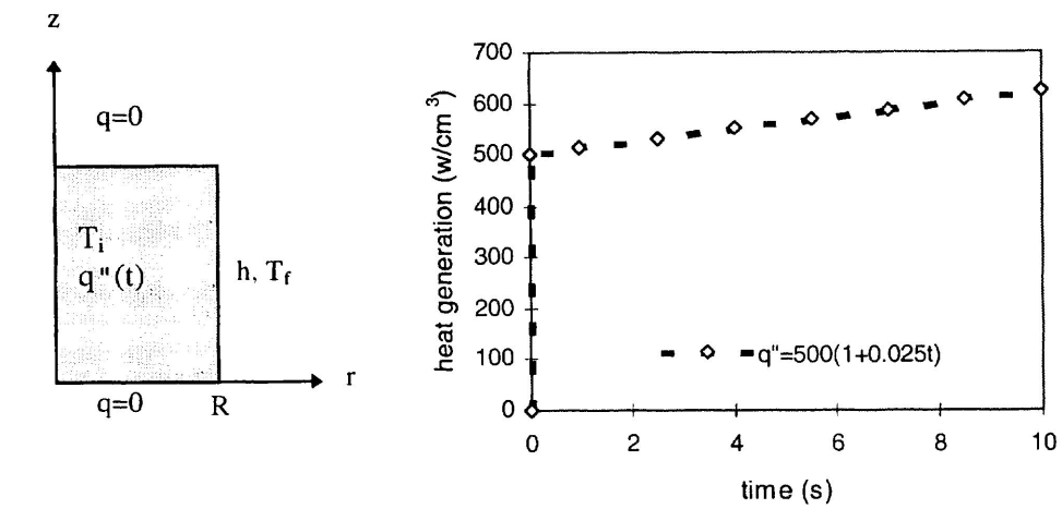
Figure 9 Heat Conduction with Time-dependent Heat Generation (Case 2-9)
