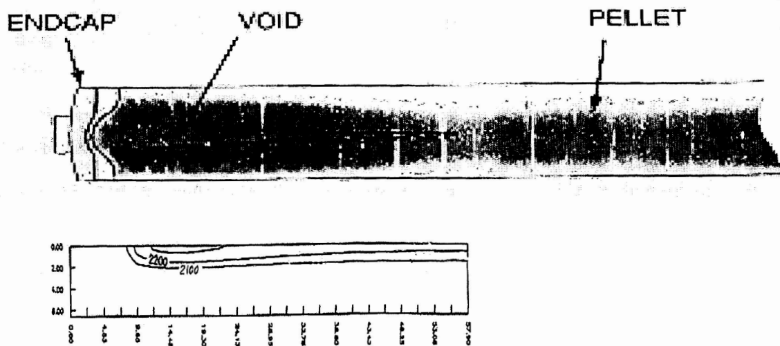
Figure 14 End-Flux-Peaking-Induced Tear-Drop-Shaped Void (top: observed, bottom: predicted) case 3-2
