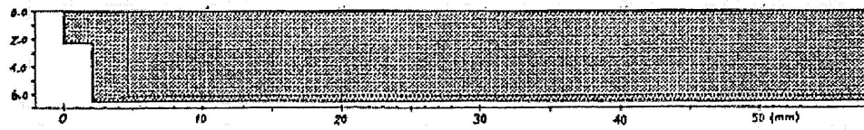
Figure 11 Finite-element Mesh Used for Case 2-14
