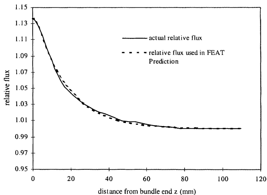
Figure 15 End Flux Peaking Profile
