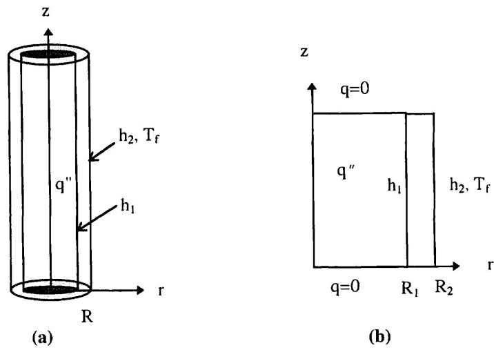
Figure 5 Heat Transfer in Two Concentric Cylinders (Case 1-6)
