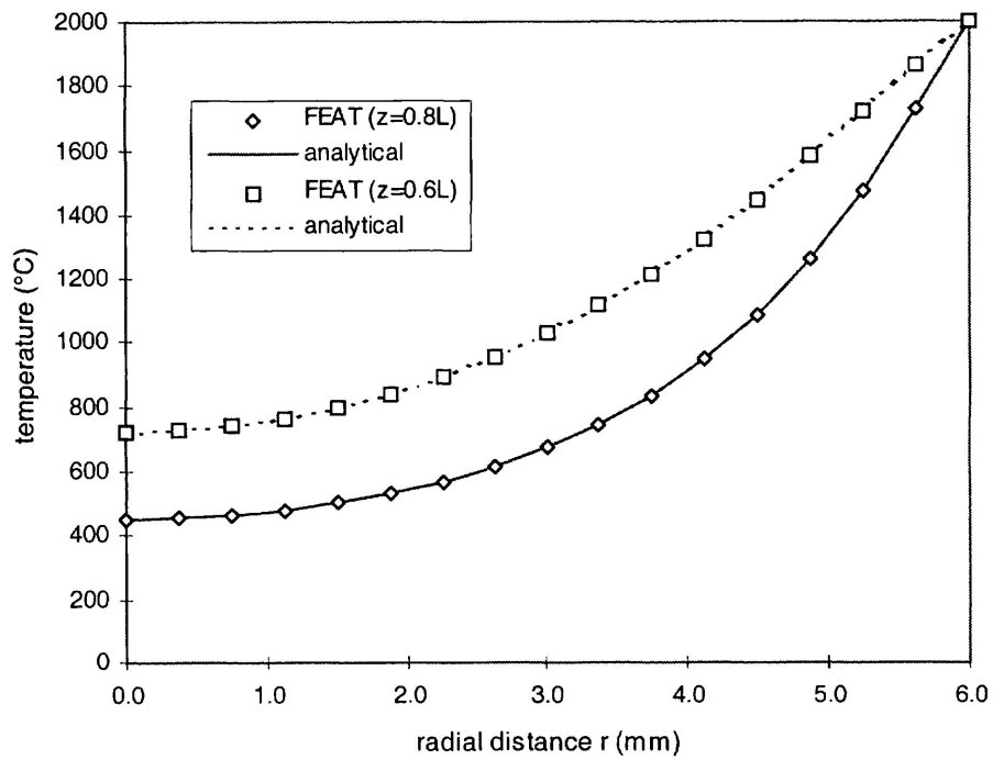
Figure 4 Two-dimensional Temperature Distribution (Case 1-3)
