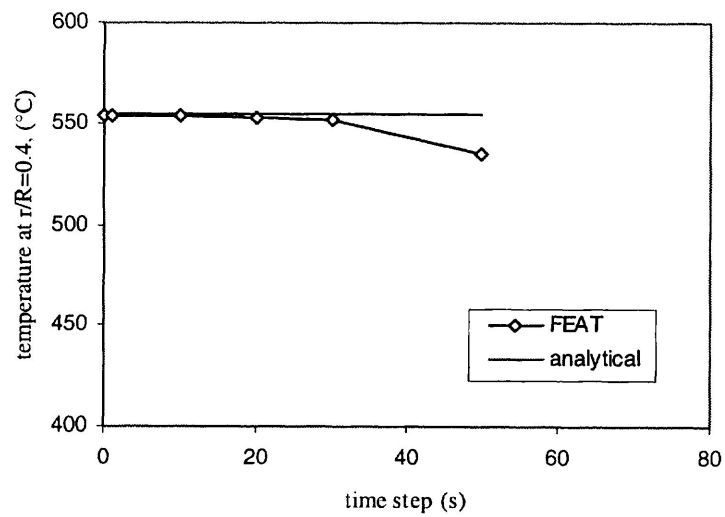
Figure 2 Time Convergence of FEAT (Case 4-3)
