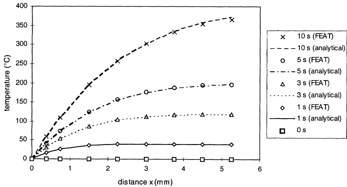
Figure 8 Temperature Profiles for Different Time Instants (Case 2-6)
