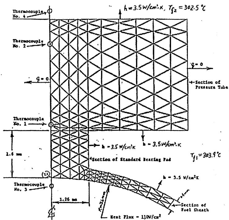
Figure 16 Thermocouple Measurement near Sheath—Bearing-Pad Interface (case 3-3)
