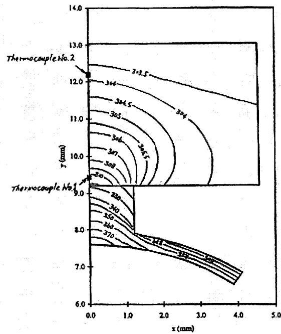
Figure 17 Predicted Isotherms near Sheath Bearing-Pad Interface
