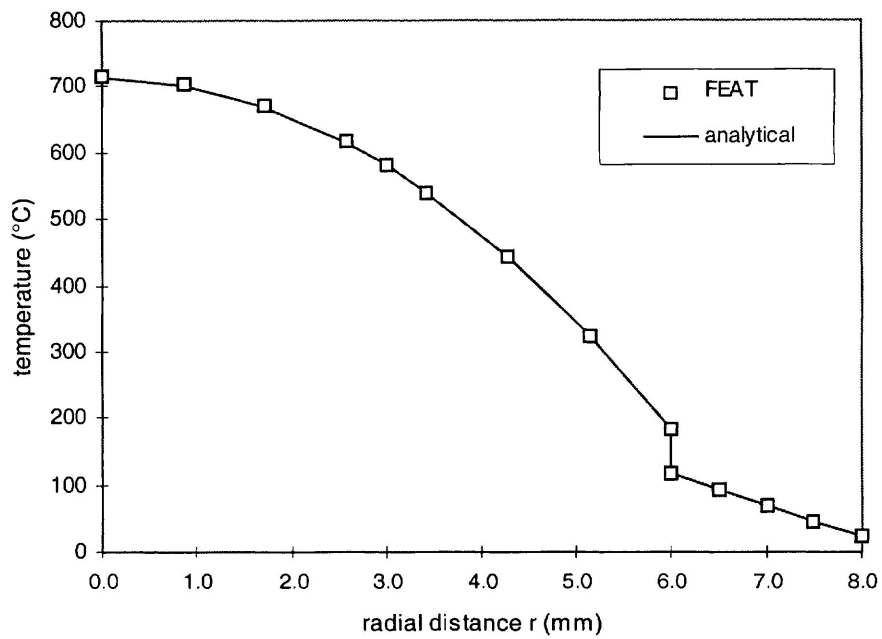
Figure 6 Temperature Profiles (Case 1-6)
