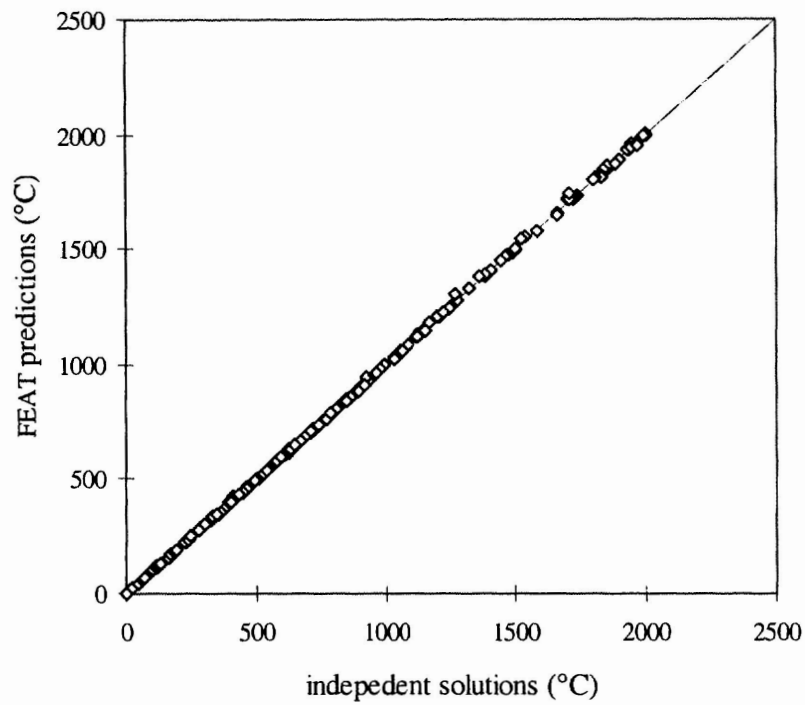
Figure 13 Overall Comparison between FEAT Predictions and Independent Solutions
