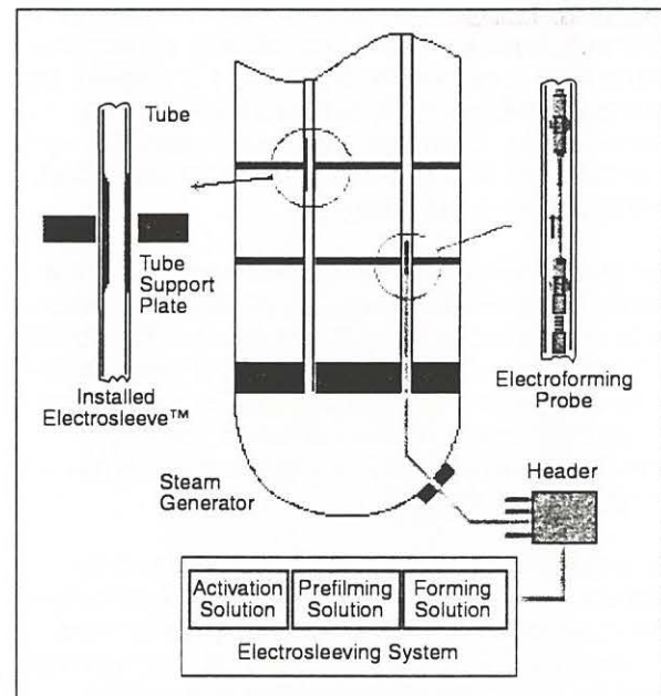
Figure 6: Simplified schematic of Electrosleeve delivery system.
