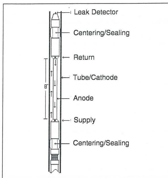
Figure 7: Schematic of plating cavity created in the SG tube by the delivery tool (probe).
