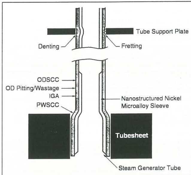
Figure 8: Electrosleeve repair of various SG degradation modes.
