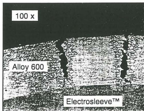
Figure 5: Cross-sectional optical micrograph showing crack arrest/blunting capability of the Electrosleeve in a stressed (2% tensile strain) Electrosleeved Alloy 600 C-ring exposed to 10% NaOH at 350°C for 3000 h.
