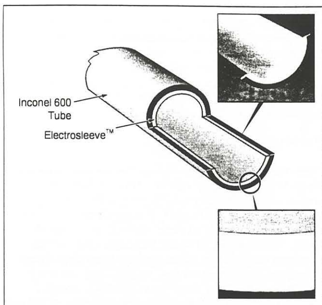
Figure 1: Cut-away view of the Electrosleeve installed in SG tubing.
