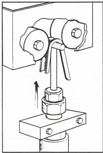
Figure 3: Reverse U-bend test of longitudinally split Electrosleeve sample.
