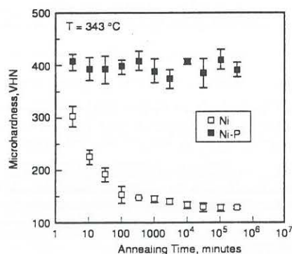
Figure 2: Vickers hardness vs. annealing time at 343°C for nanocrystalline (1) Ni and (2) Ni-1500 ppm P.
