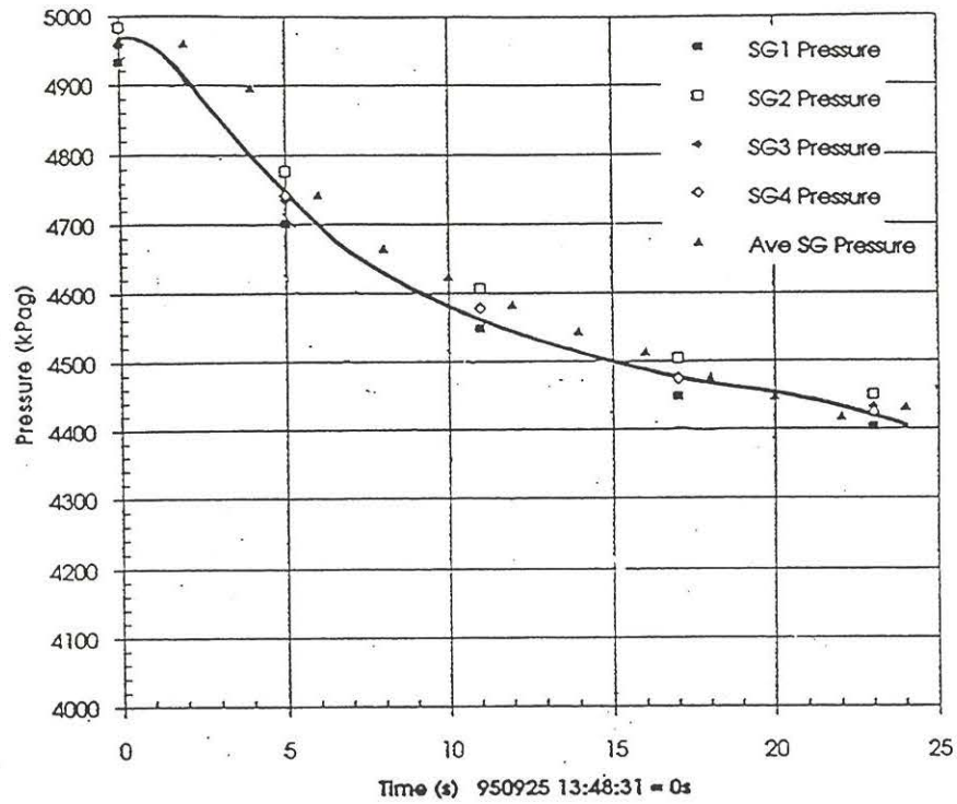
Figure 4. Comparison of steam drum pressure at SG2 (at NE) with plant data
