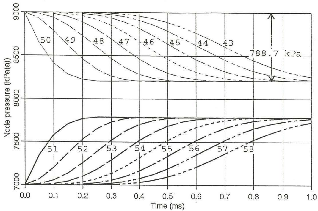
Figure 1c. TUF Simulation - Long pipe with moving plate Pressure transient
