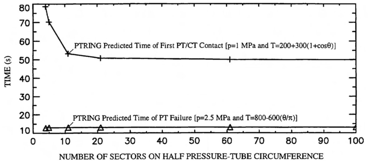
FIGURE 2: Influence of Total Number of Sectors on PTRING Results in Two Numerical Tests (Each Sector was Divided into 10 Subsectors in PTRING)
