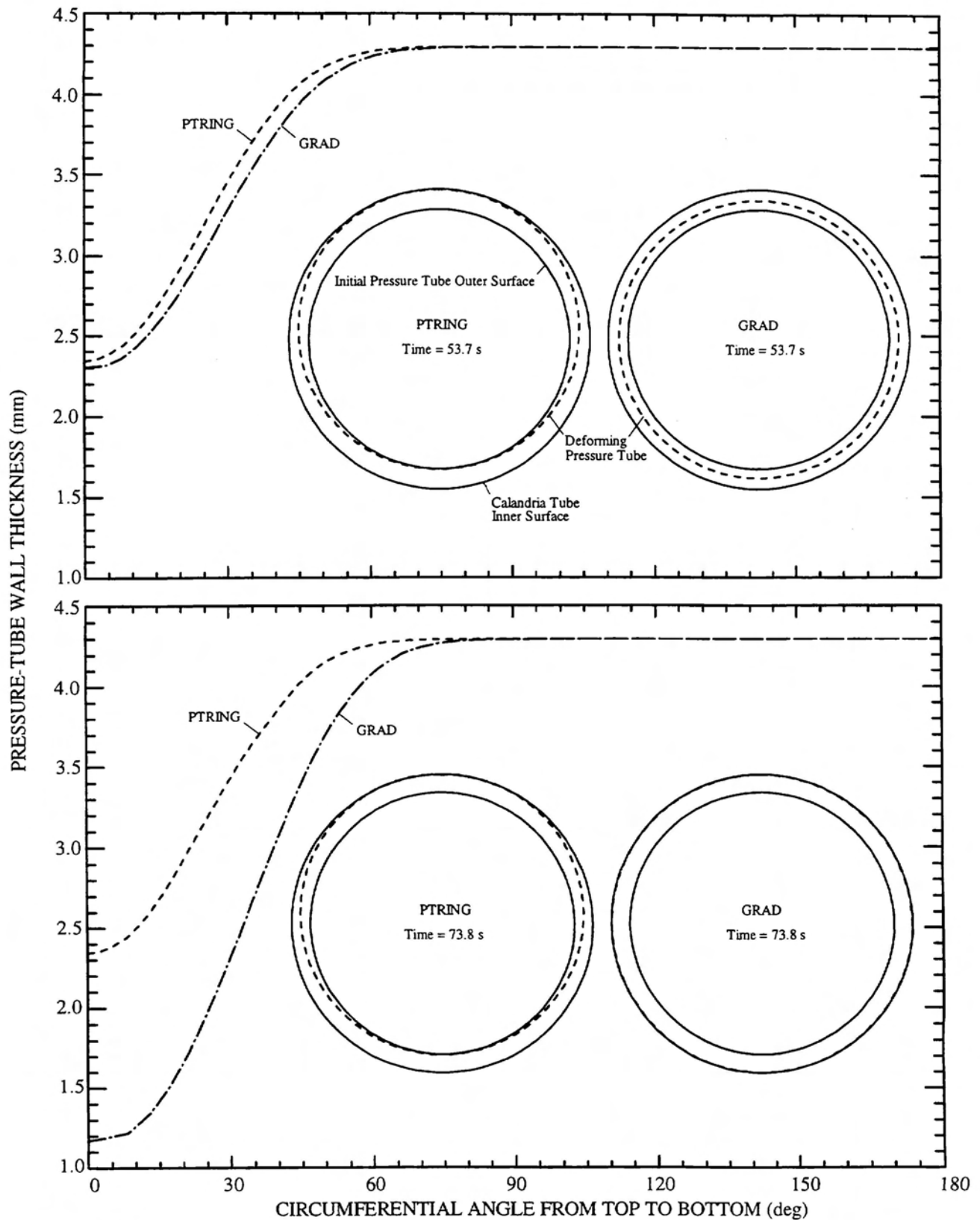
FIGURE 3: Comparison Between the Circular and Noncircular Models on Predicted Pressure-Tube Geometry and Circumferential Wall Thickness Distribution at Two Different Times ( T=200+300(1+\cos\theta) ; p=1 MPa)
