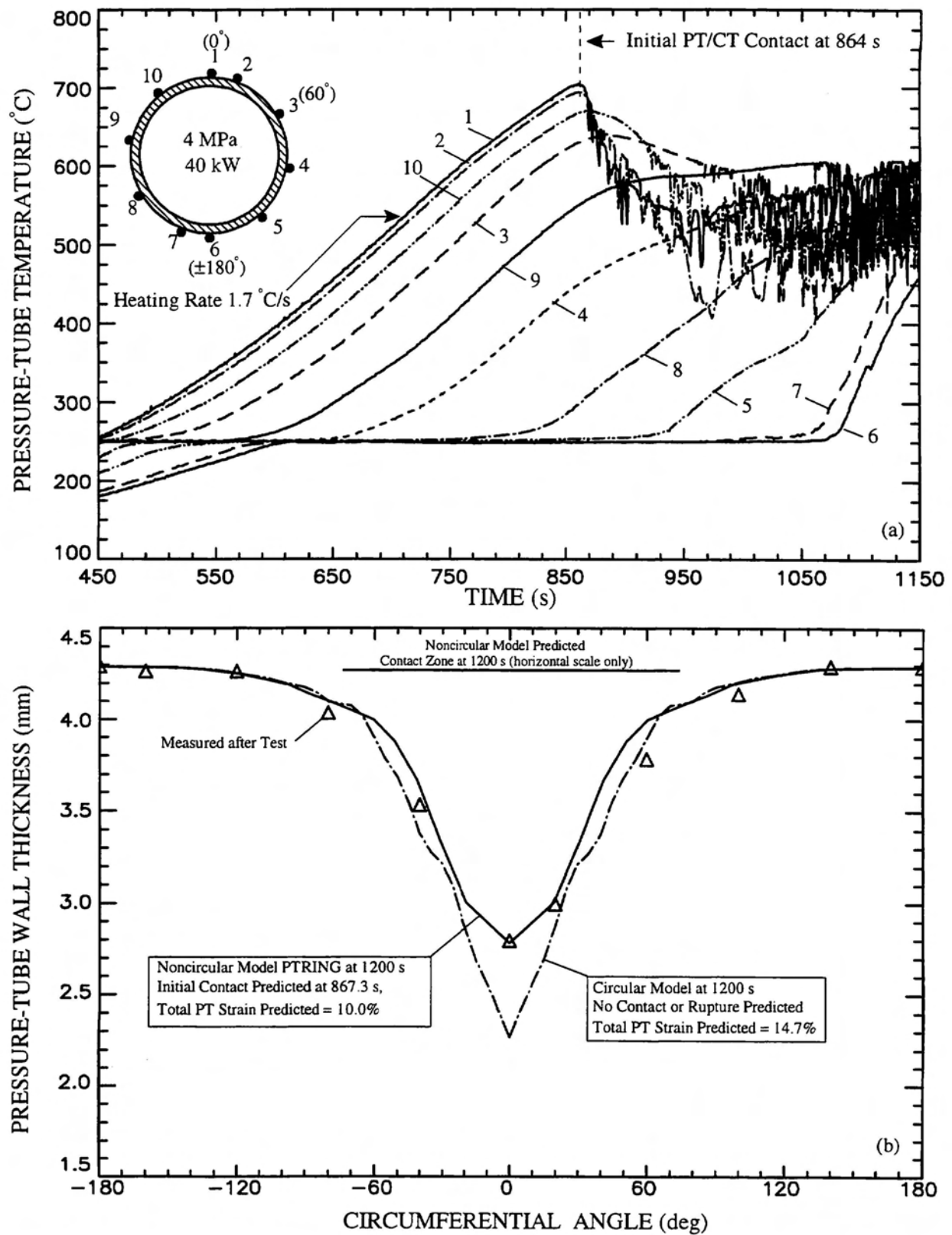
FIGURE 4: Measured Pressure-Tube Outer-Surface Temperatures (a) and Measured and Predicted Pressure-Tube Wall Thicknesses (b) at Axial Location 2 of PTΔT Test S-1-4
