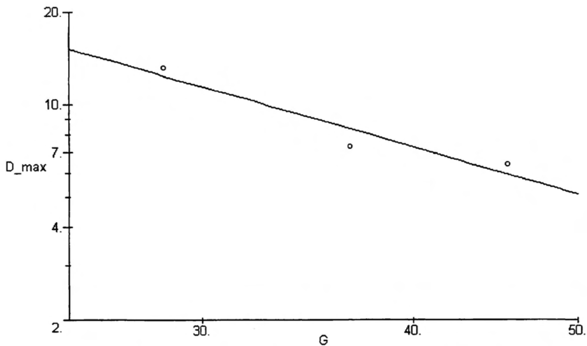
Figure (3): Maximum cluster size, microns, versus turbulent shear gradient, s^{-1} . Results for silica powder.
